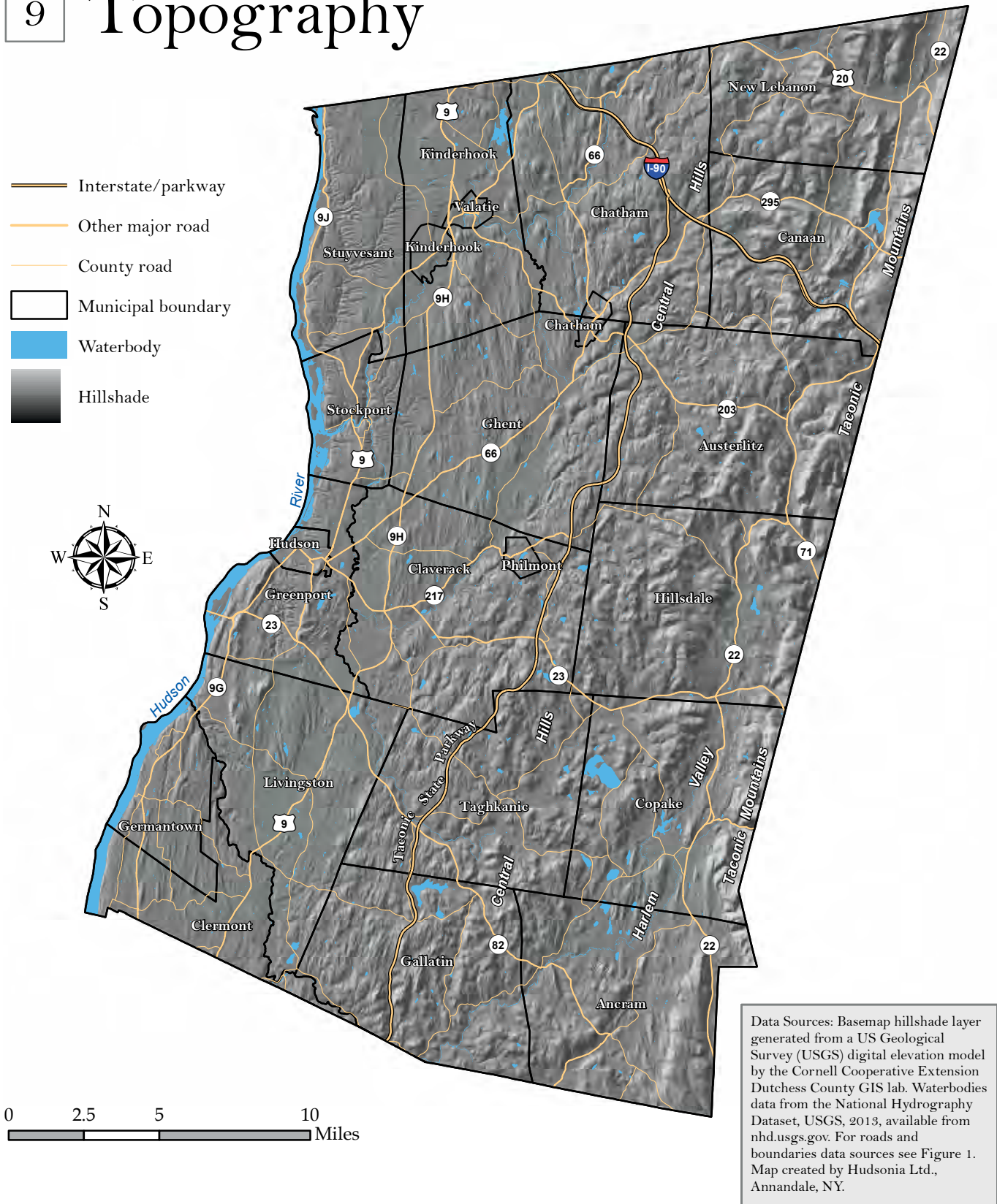
Figure 9. Topography of Columbia County, New York. Columbia County Natural Resources Inventory, 2018.
